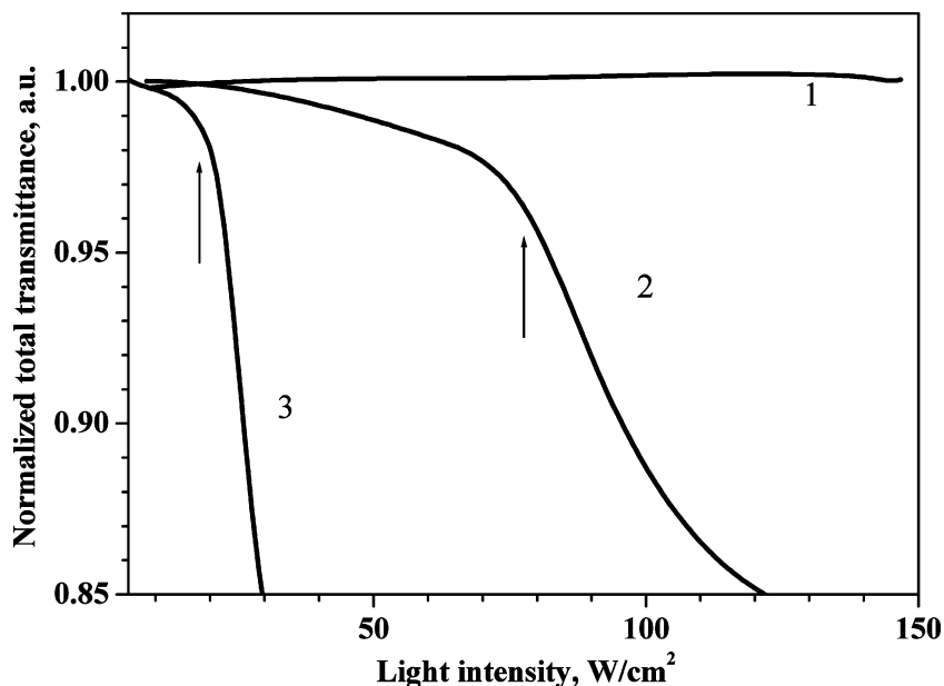
FIGURE 2 Total transmittance (normalized on the linear transmittance) of a 10\text{ }\mu\text{m} homeotropic cell vs. I for different c : 1 – pure 5CB, 2 – 0.68 wt.%, 3 – 1.4 wt.%. Arrows show the thresholds of DR.
